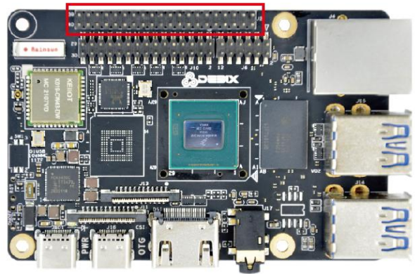
Figure 11 Pin header of DEBIX motherboard
